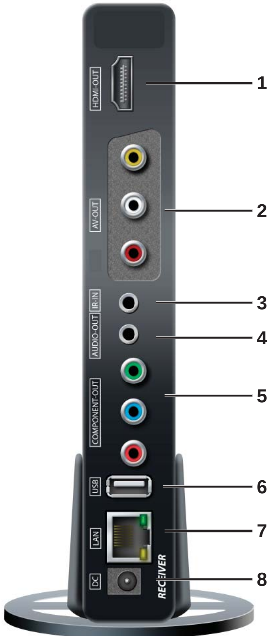
Receiver Back
