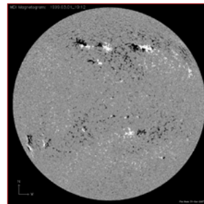
MDI Magnetogram showing Sunspot north (white) and south (black) poles. science.nasa.gov
