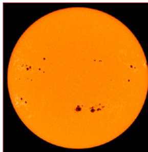
Intensitygram showing dark Sunspots umbra.nascom.nasa.gov
